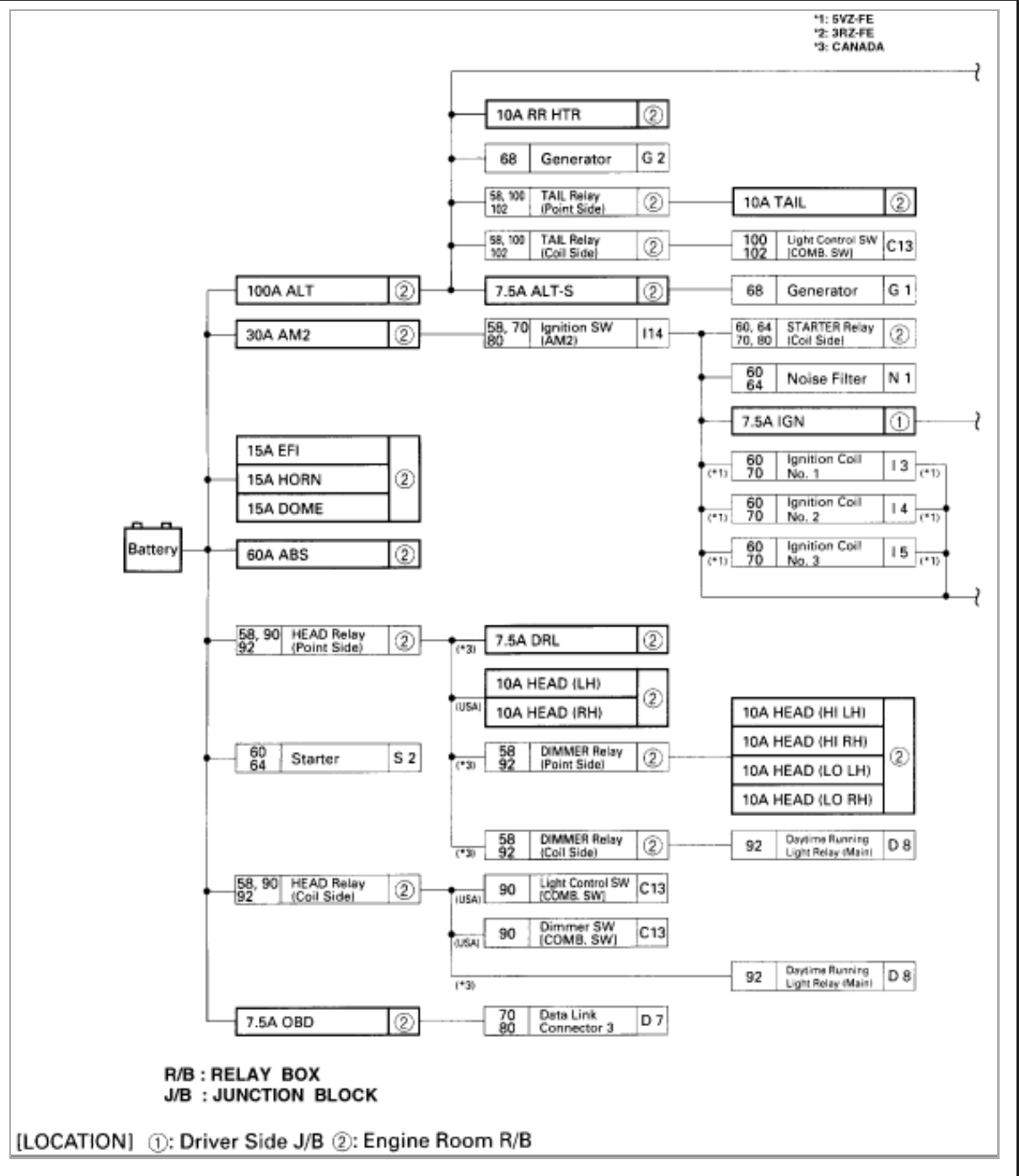
Power Source (Current Flow Chart) (Part 2 Of 2)
