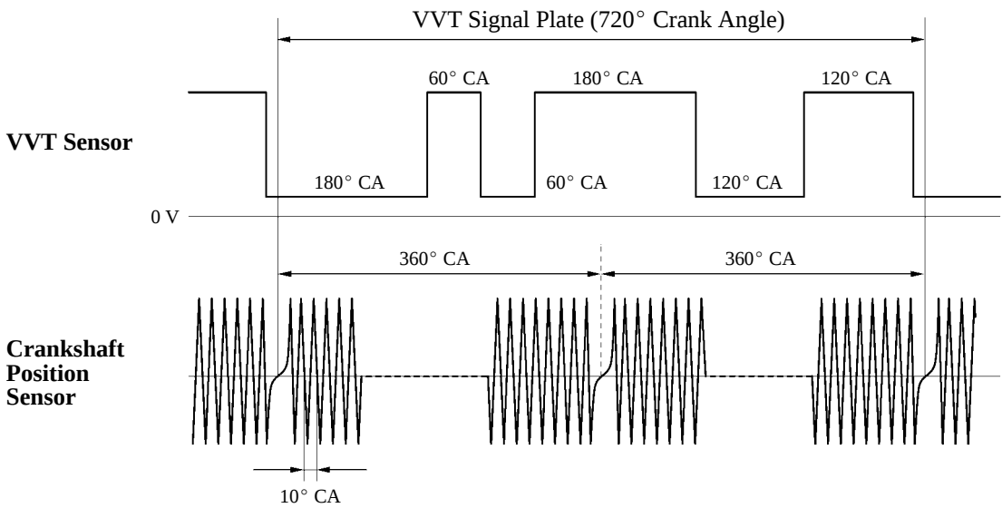
Correlation of Output Waveform between VVT Sensor and Crankshaft Position Sensor
