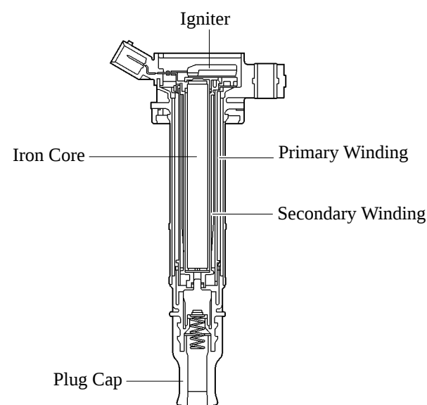
Ignition Coil Cross Section
