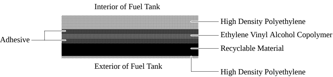
Cross Section of Fuel Tank
