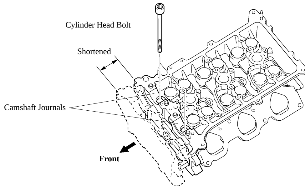
Right Bank Cylinder Head
