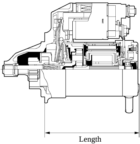
PS Type Starter
