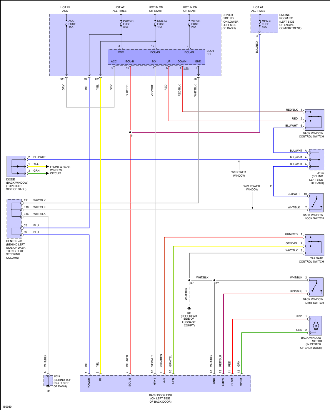
Fig 2: Tailgate Power Window Circuit
