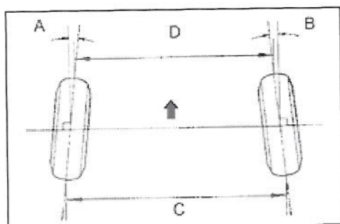
Standard Toe-in (Unloaded Vehicle):
