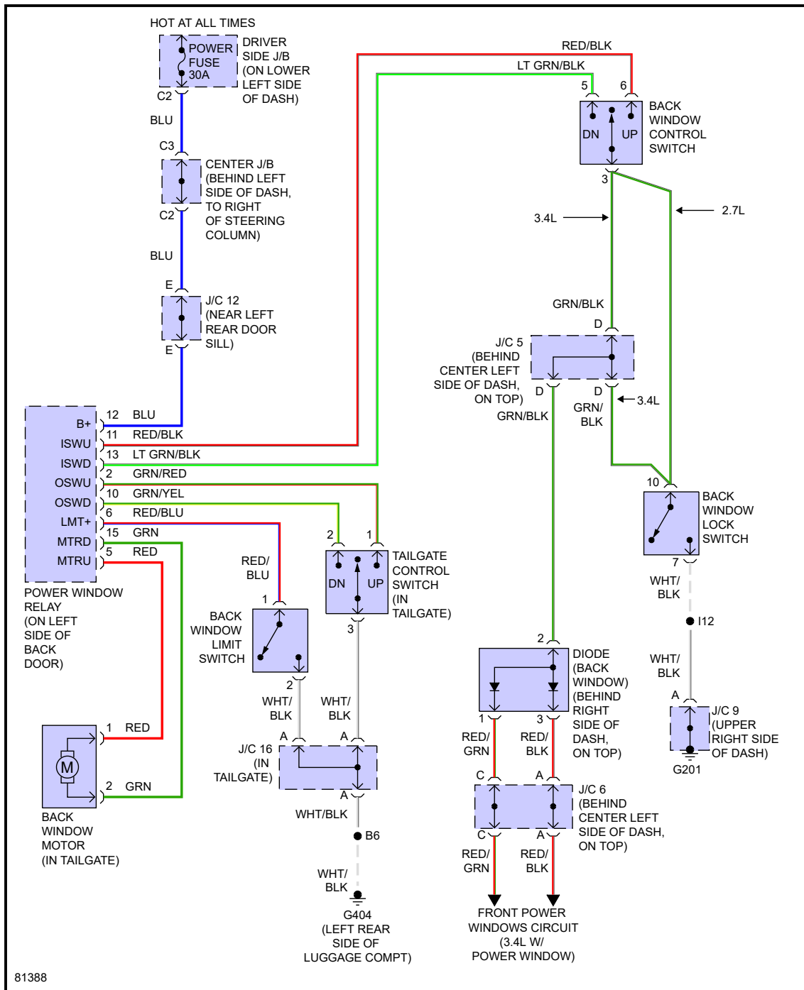
Fig 2: Power Windows Circuit, Rear
