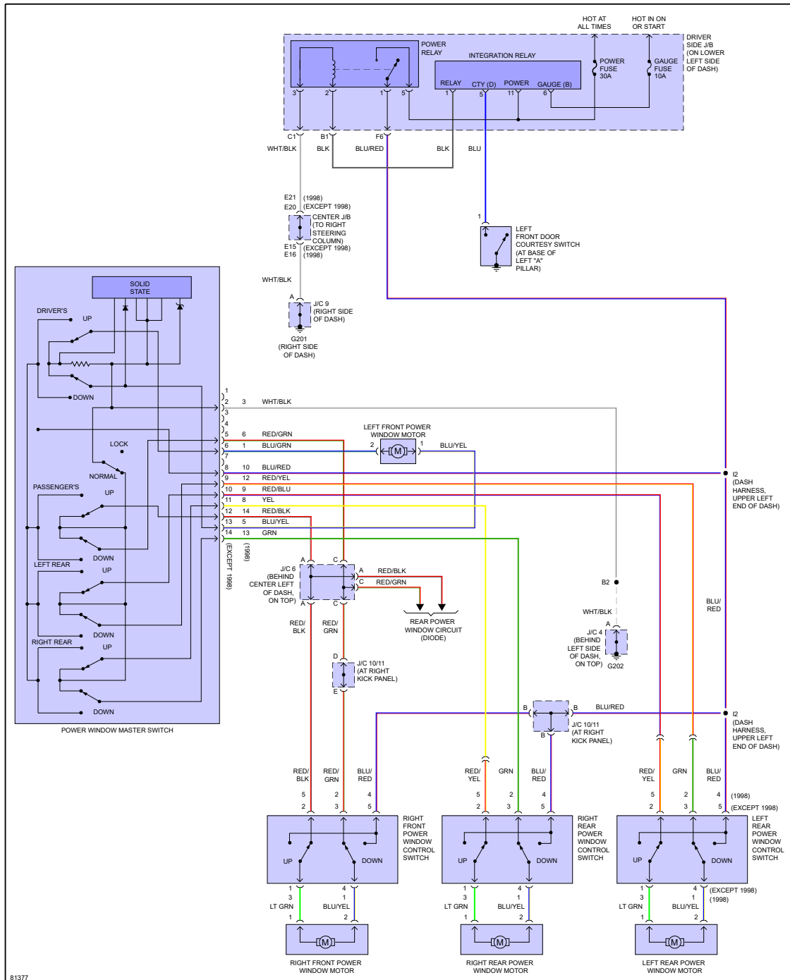
Fig 1: Power Windows Circuit, Front
