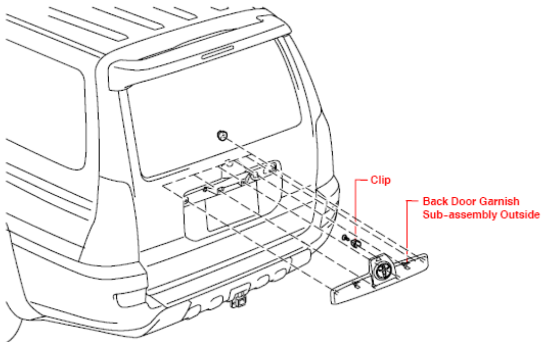
Fig. 2: Installing Back Door Outside Garnish Sub-Assembly Courtesy of TOYOTA MOTOR SALES, U.S.A., INC.
