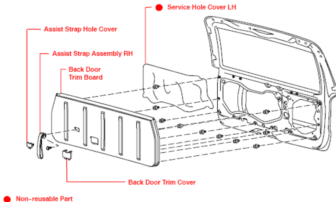
Fig. 1: Removing Back Door Garnish Sub-Assembly Courtesy of TOYOTA MOTOR SALES, U.S.A., INC.
