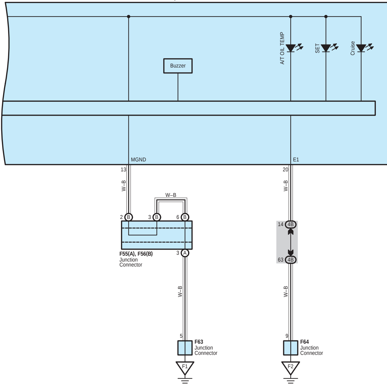
F14 Combination Meter Assembly
