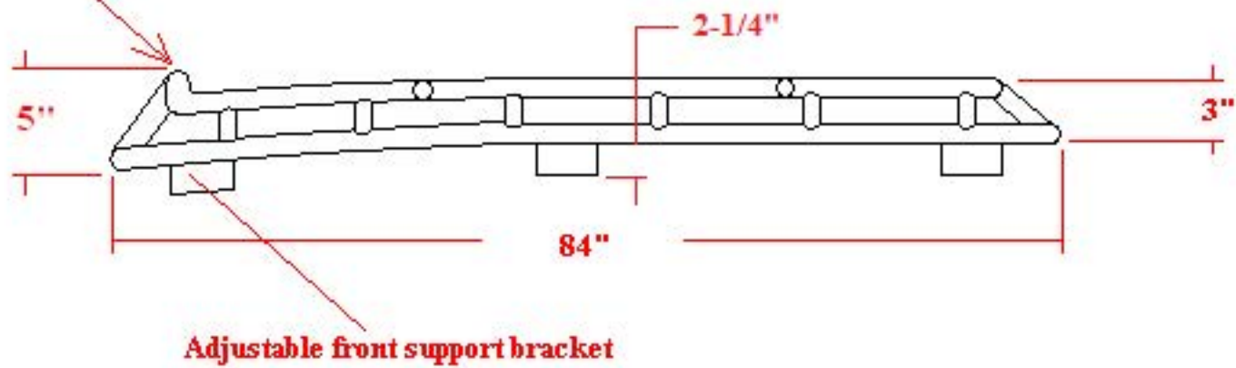
SIDE VIEW OF GOBI 4 RUNNER ROOF RACK
