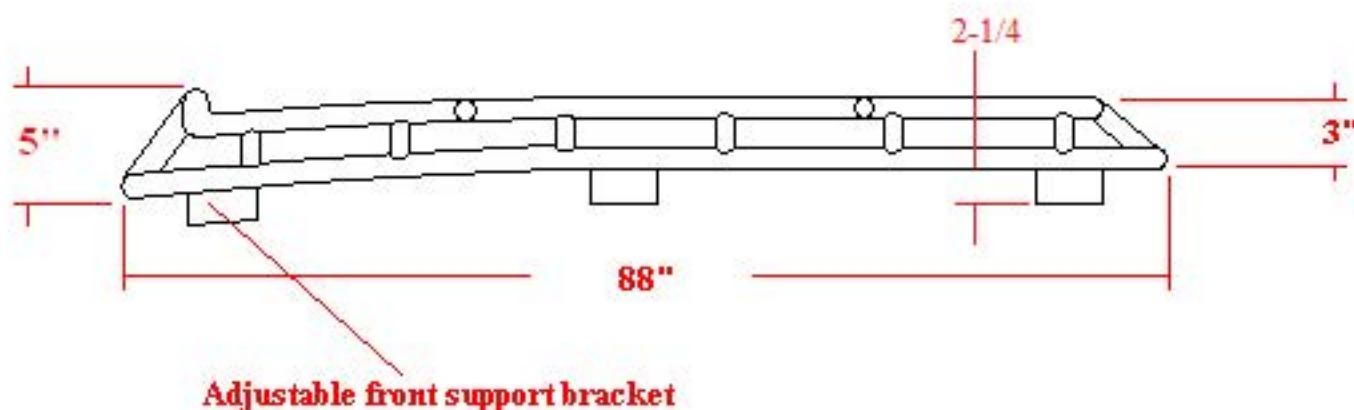
SIDE VIEW OF GOBI 2010 4 RUNNER ROOF RACK
