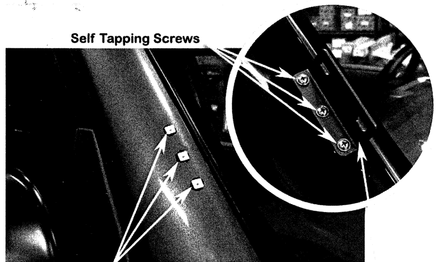
Plastic Inserts
