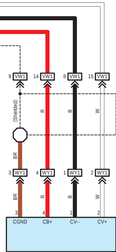
Y1 Rear Television Camera Assembly
