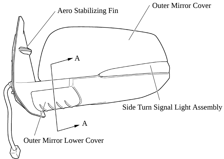
Outer Rear View Mirror Assembly
